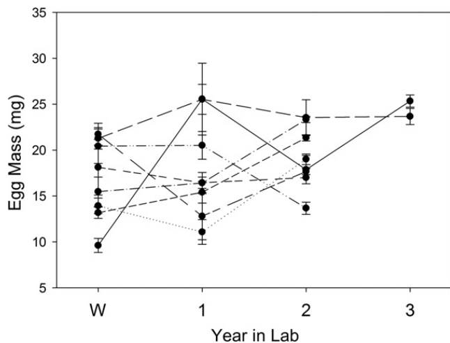
Fig. 2. Mean ( \pm SE) mass (mg) of eggs from eight female newts ( Taricha granulosa ) from initial collection in the wild (W) through three additional years in captivity. There was no significant change in egg mass between years ( F_{(3,15)} = 2.15 , P = 0.136 ).
