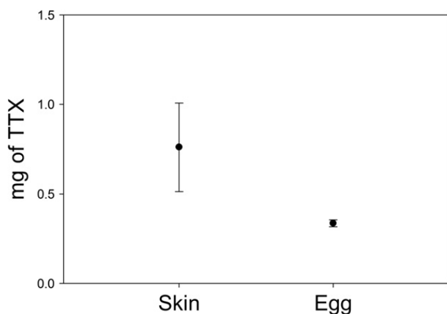
Fig. 3. Comparison of the mean ( \pm SE) amount of TTX regenerated in the skin of adult newts ( Taricha granulosa ) over 9 months (Skin) versus the estimated mean ( \pm SE) amount of TTX provisioned by eight female newts in an entire clutch of 525 eggs (Eggs). Regenerated skin TTX was calculated by estimating whole-body TTX from raw data in Cardall et al. (2004) and subtracting post-stimulus TTX from final TTX. An estimate of the total TTX provisioned in a clutch of eggs for each female reared in captivity was calculated by multiplying the average egg toxicity from years one, two, and three for each female by 525 [the average number of eggs produced by females from our study site (Hanifin et al., 2003)]. These values were then averaged to obtain an estimate of the amount of TTX ( \pm SE) provisioned in an entire clutch of eggs in the laboratory. In both studies (Cardall et al., 2004; this study) the newts were fed a TTX-free diet. There is no significant difference between the amount of TTX regenerated in the skin and the amount of TTX provisioned in a clutch of eggs by newts in the laboratory (Mann–Whitney: U = 223 , P = 0.25 ).
