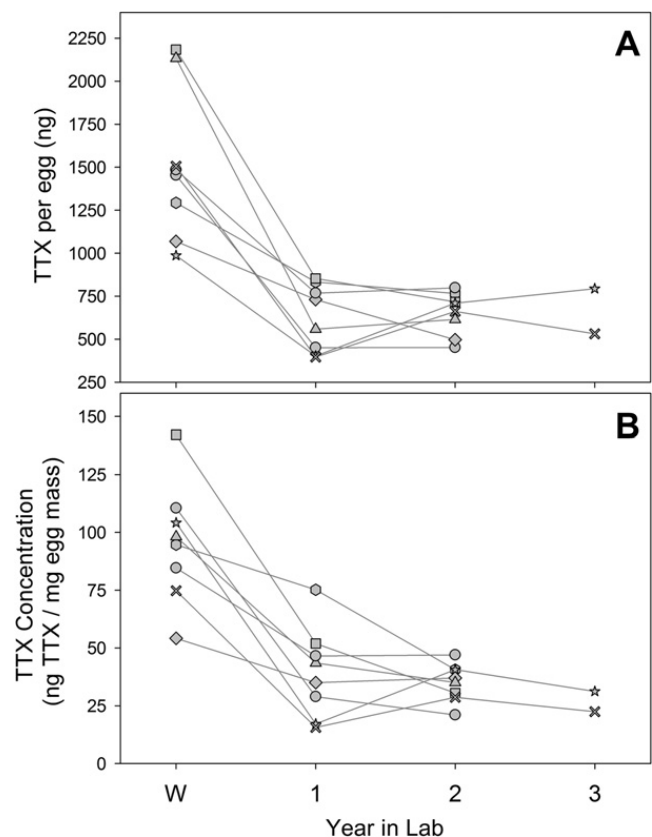
Fig. 1. Mean total TTX (A) and TTX concentration (ng TTX/mg egg mass) (B) present in eggs from eight different female Taricha granulosa . A sample of eggs was taken immediately after collection from these wild-caught females (W), and after one, two, and three years in captivity. There was a significant decline in total TTX ( F_{[3,15]} = 32.7 , P < 0.0001 ) and TTX concentration ( F_{[3,15]} = 34.8 , P < 0.0001 ) after the first year in captivity, yet substantial quantities of toxin were present and remained relatively constant in the following three years.
